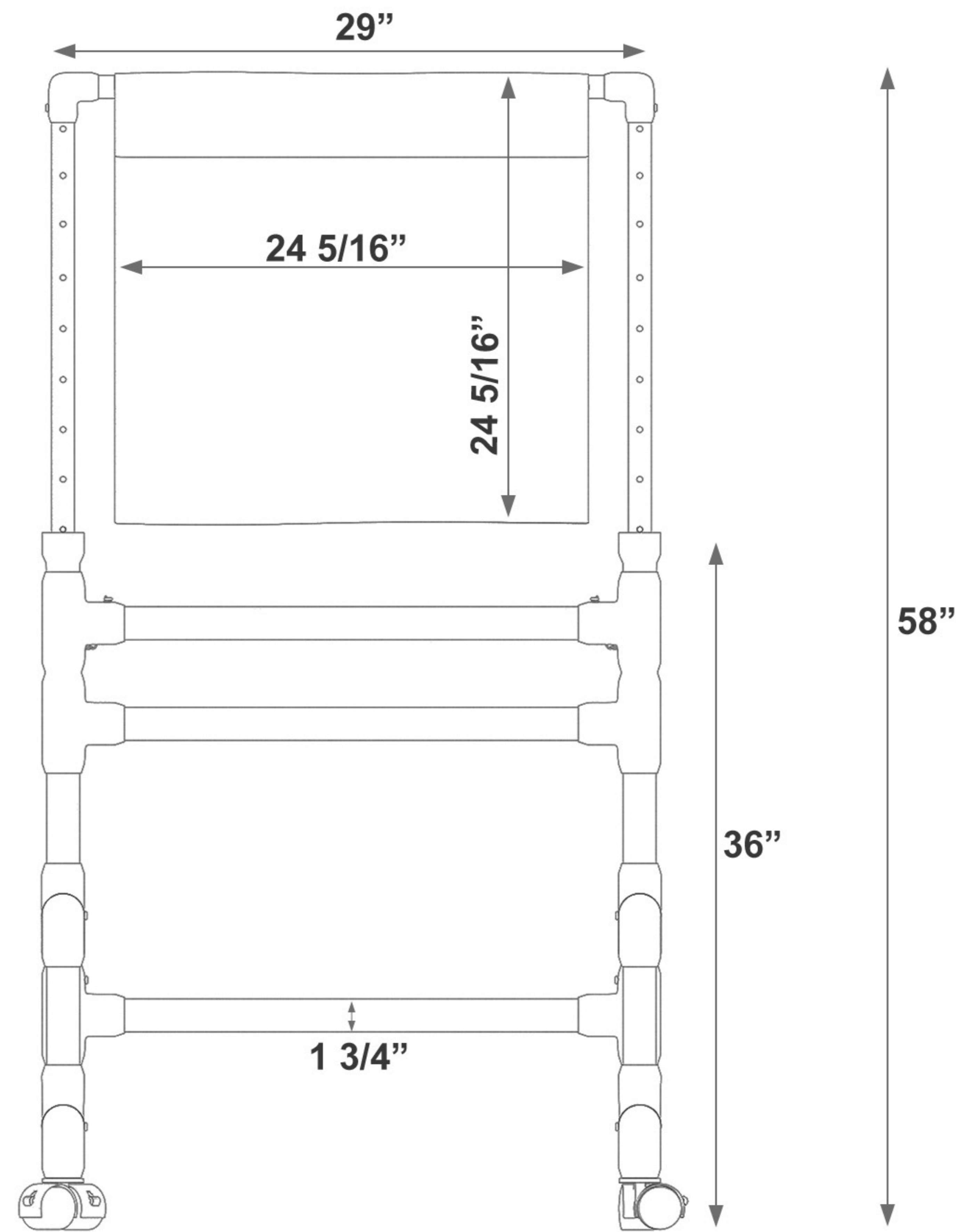
BACK VIEW
