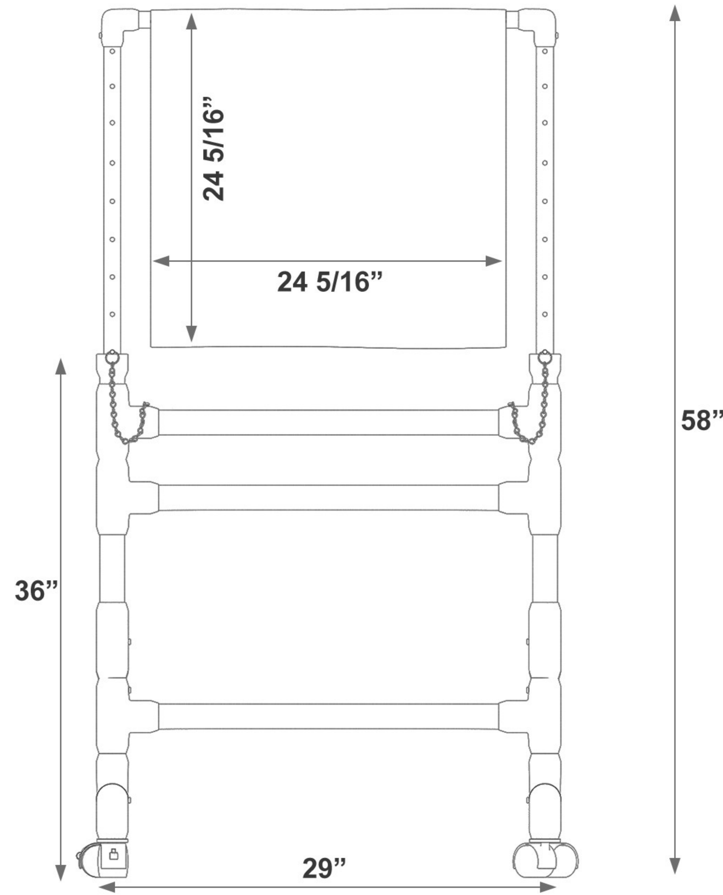
FRONT VIEW
