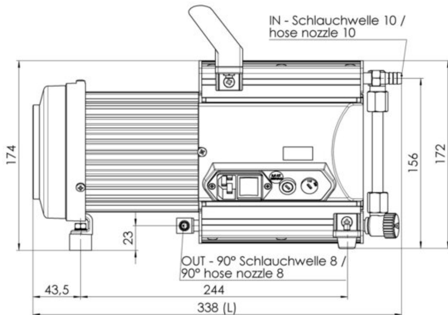
VACUUBRAND MD 1C Version 03
