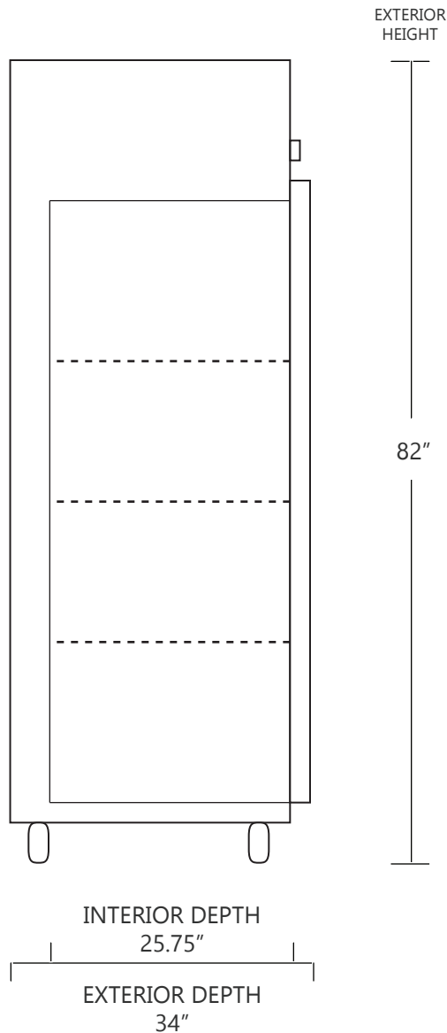
SIDE VIEW
