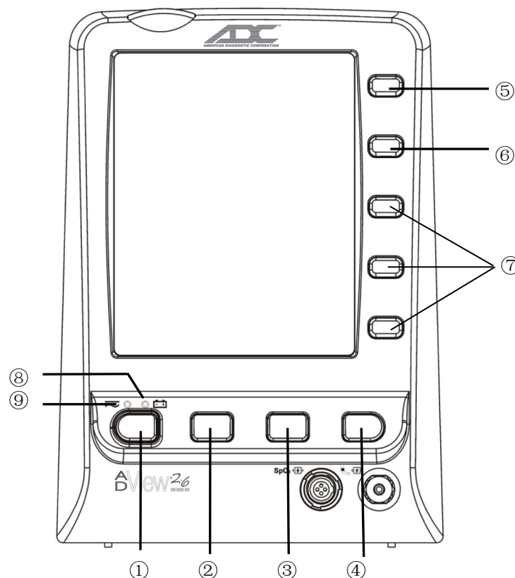
Figure 3-10 Buttons
