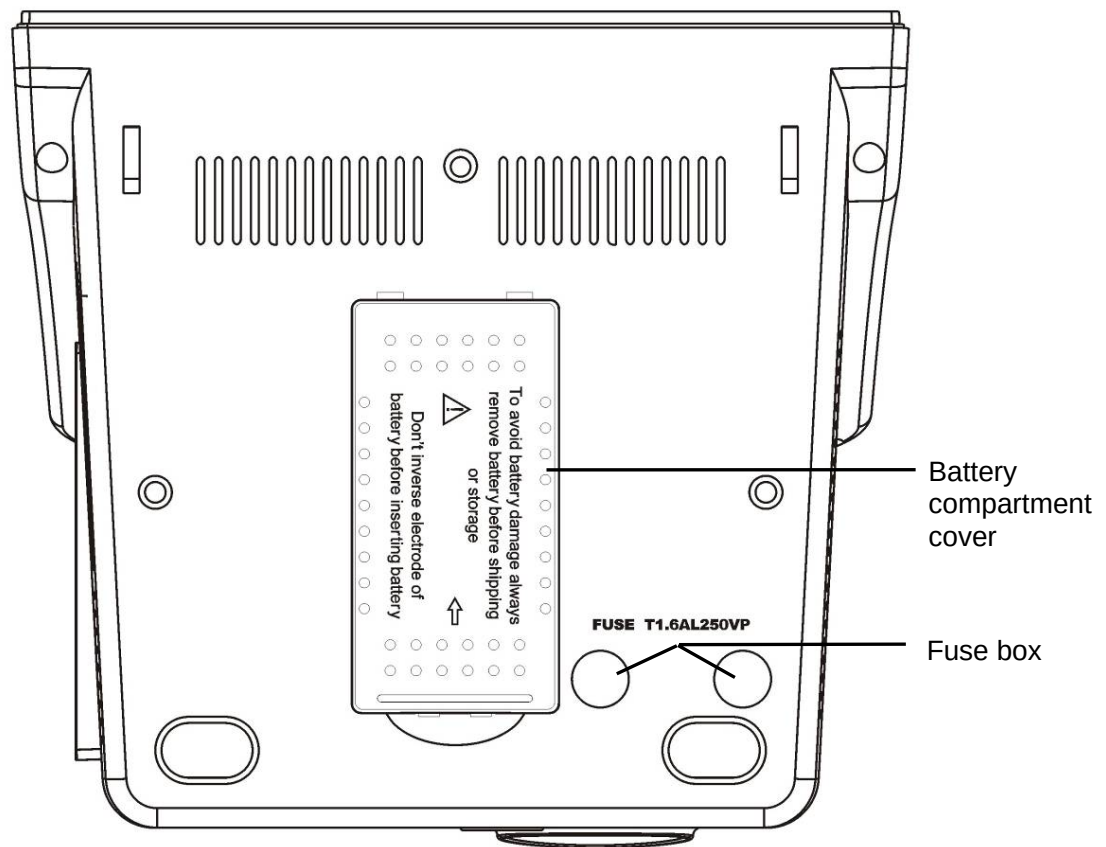
Figure 3-14 Bottom panel
