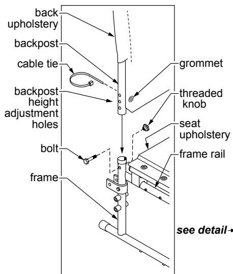
Adjustable Back pre-installation, right side (right arm, right rear wheel, and crossbraces not shown)
