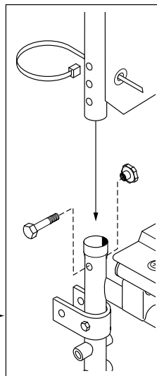
Pre-installation detail
