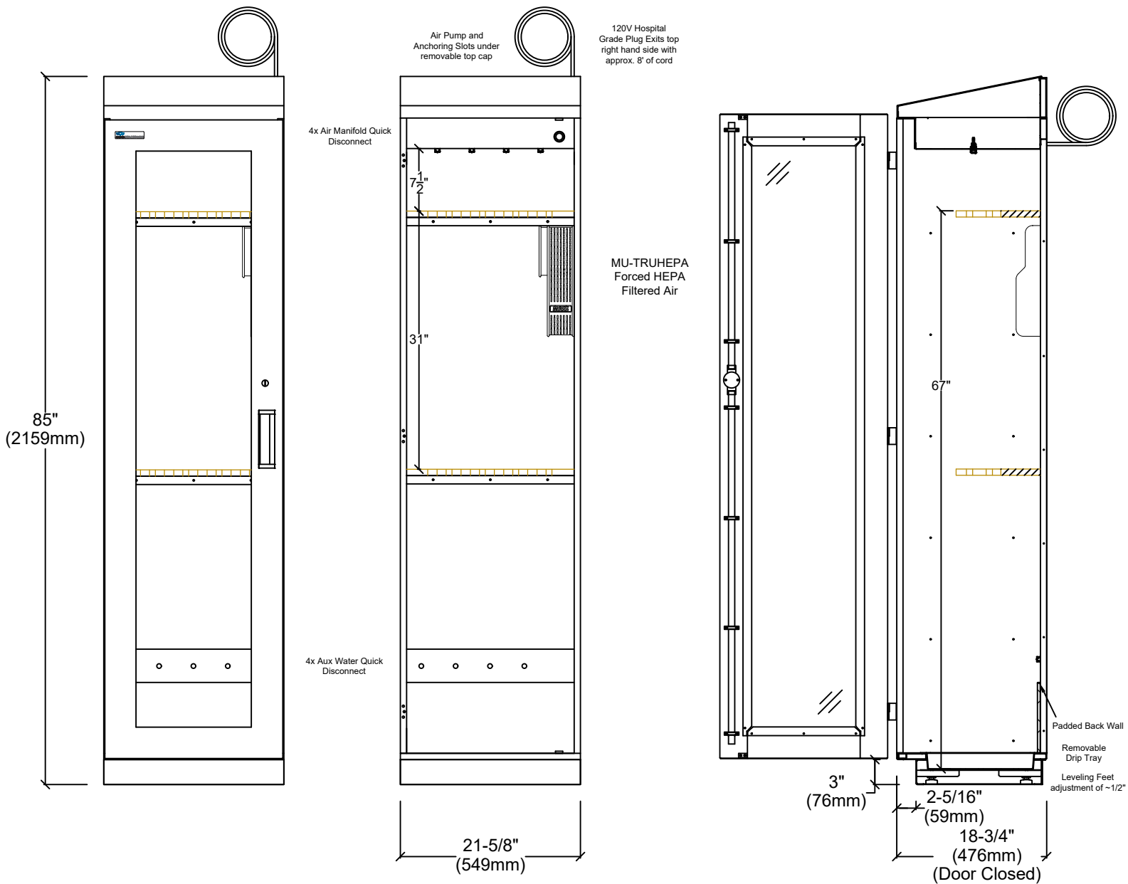
Item POWDER-COATED METAL SAS-B04P-ENT-DRY SCOPE DRYING CABINET Locking Overlay Hinged Door with Glass Insert
