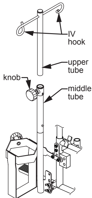
step 2: Install IV hanger
