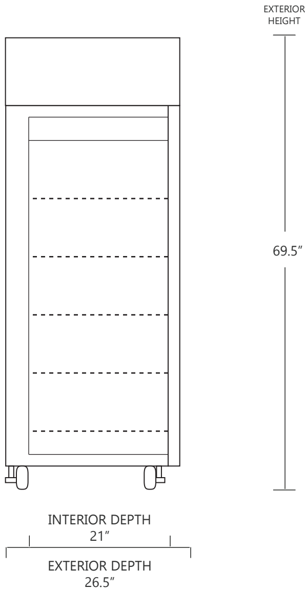
SIDE VIEW
