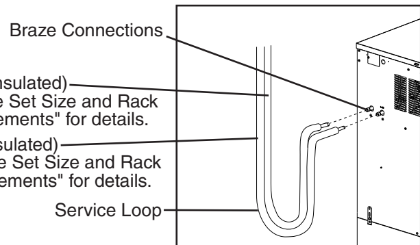
Icemaker Braze Connection
