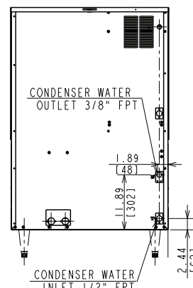
DCM-751BWH-OS WATER-COOLED
