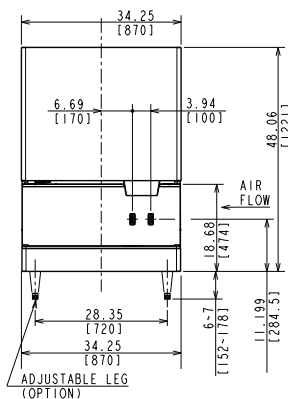
DCM-752BAH-OS AIR-COOLED
