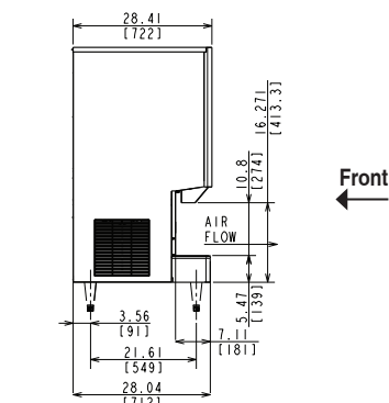
DCM-752BAH-OS AIR-COOLED
