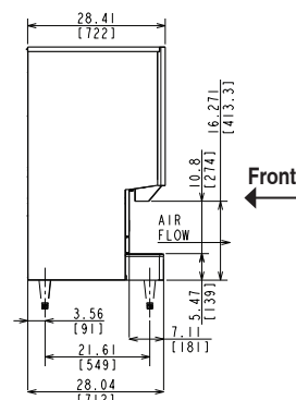
DCM-751BWH-OS WATER-COOLED
