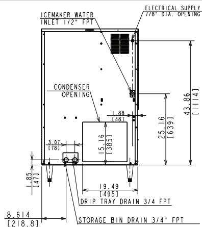
DCM-752BAH-OS AIR-COOLED
