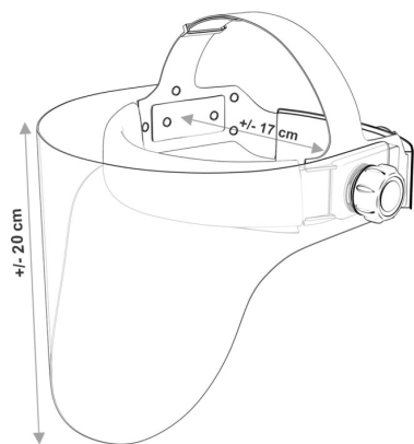
PERSPECTIVE VIEW
